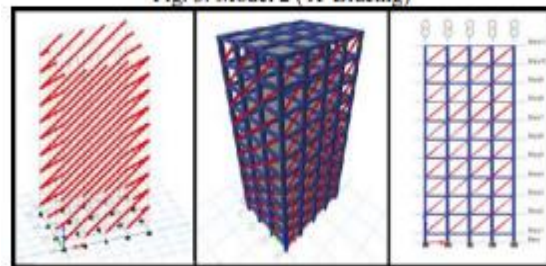
Fig. 4: Model 3 (Diagonal Bracing)
