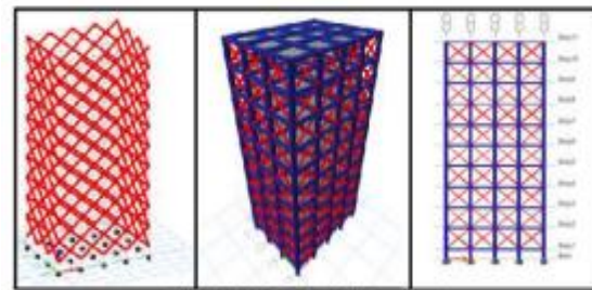
Fig. 3: Model 2 ('X' Bracing)
