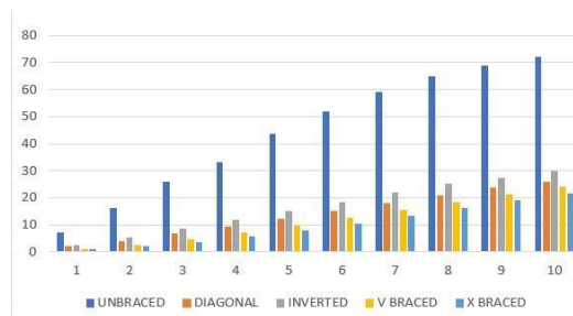
Fig 11 . Story Drift in Y – Direction
