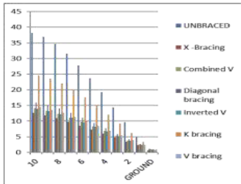
Fig 8. Maximum Lateral Displacement (mm) in X Direction
