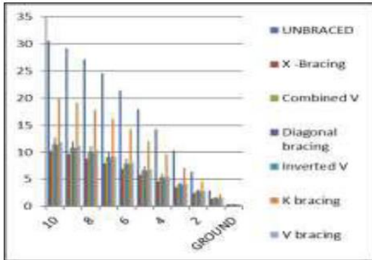
Fig 8. Maximum Lateral Displacement (mm) in X Direction
