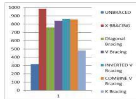
Fig 13. Base shear in X- Direction
