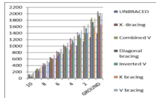
Fig 12. Axial forces
