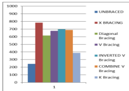
Fig 14. Base shear in Y- Direction
