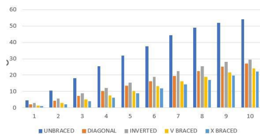
Fig 10. Story Drift in X – Direction
